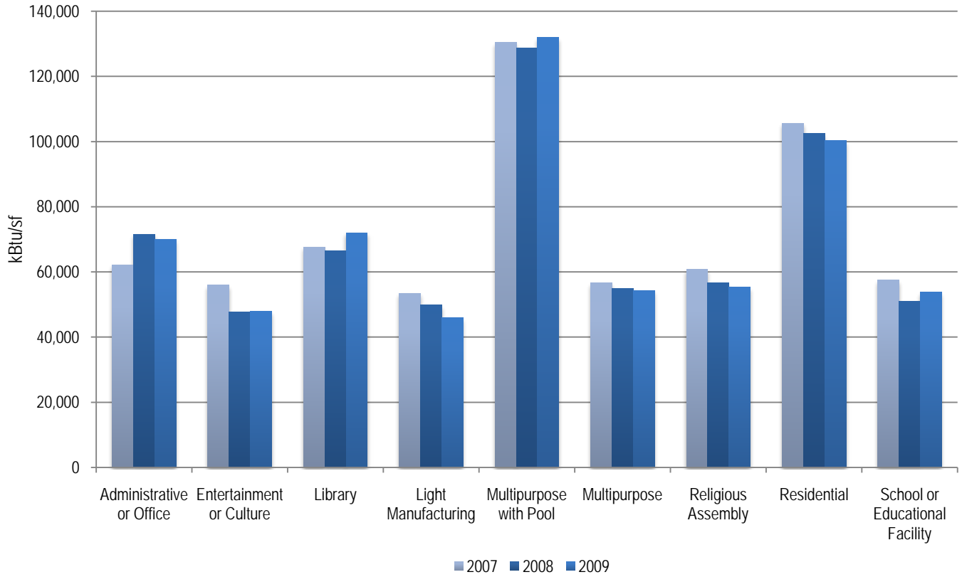
Energy Use Per Square Foot By Category
